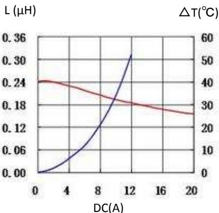
2. 0512CDMCCDS-R22MC
