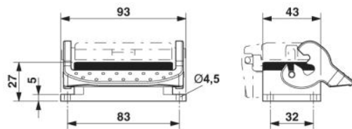
Dimensional drawing
