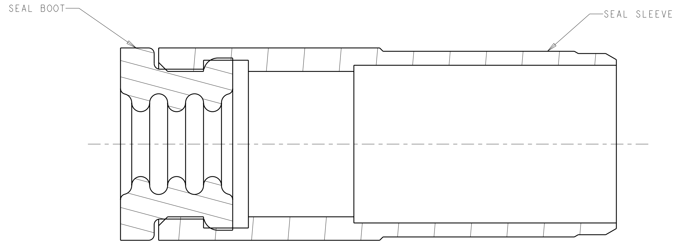
SECTION J-J
