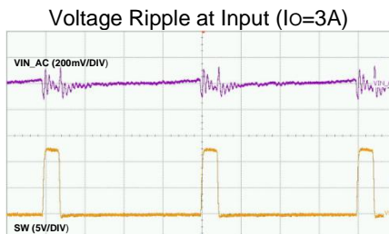
Time-400ns/div
