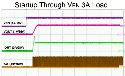
Time-1ms/div
