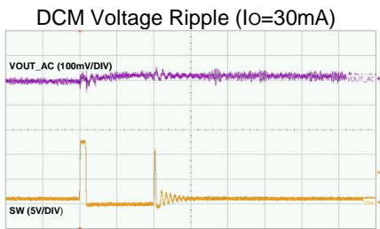
Time-1μs/div
