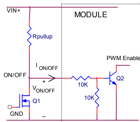
Figure 43. Circuit configuration for using negative On/Off logic.
