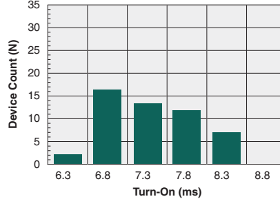
Typical Turn-On Time (N=50, I F =20mA, I L =1A DC )
