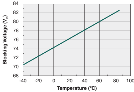
Normalized Blocking Voltage vs. Temperature
