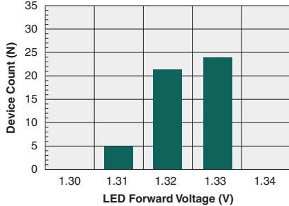
Typical LED Forward Voltage Drop (N=50, I F =10mA, I L =1A DC )
