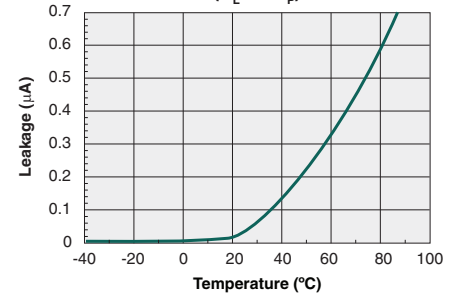
Typical Leakage vs. Temperature Measured Across Pins 1&2 ( V_L=60\text{V}_p )
