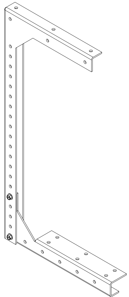
ISOMETRIC VIEW
