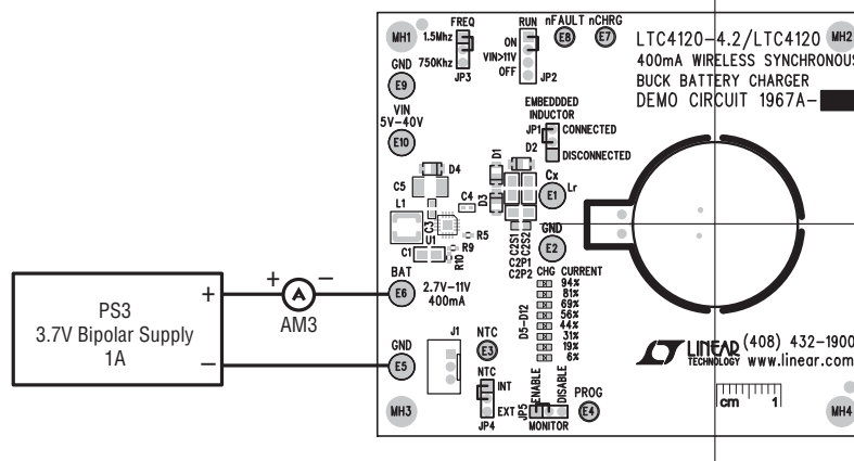
Figure 7c. Receive Board with Battery Emulator
