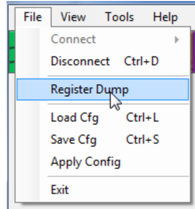
Figure 22. Dumping Registers
