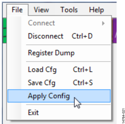
Figure 21. Apply Configuration
