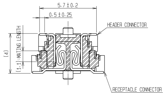
CROSS CUT SECTION - SIGNAL (5:1)
