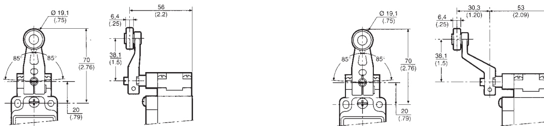
Side Rotary Roller Lever A1A Plastic Roller A1B Metal Roller
