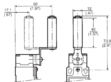
Side Rotary Conveyor Lever A9A Ceramic Roller
