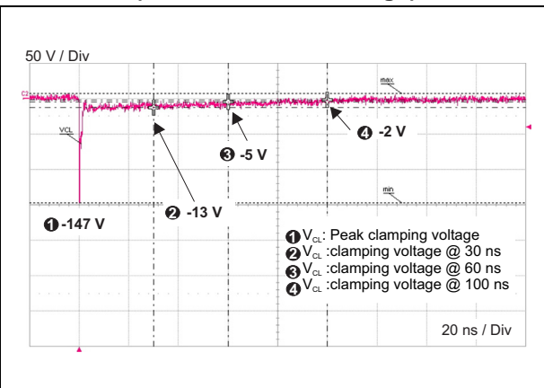
Figure 13. ESD response to IEC 61000-4-2 (-8 kV contact discharge)
