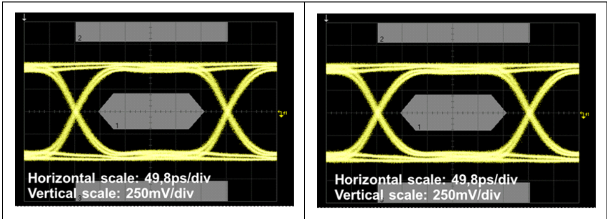
Figure 4. Eye diagram - HDMI mask at 3.4 Gbps per channel (without HSP051-4N10) (1)
