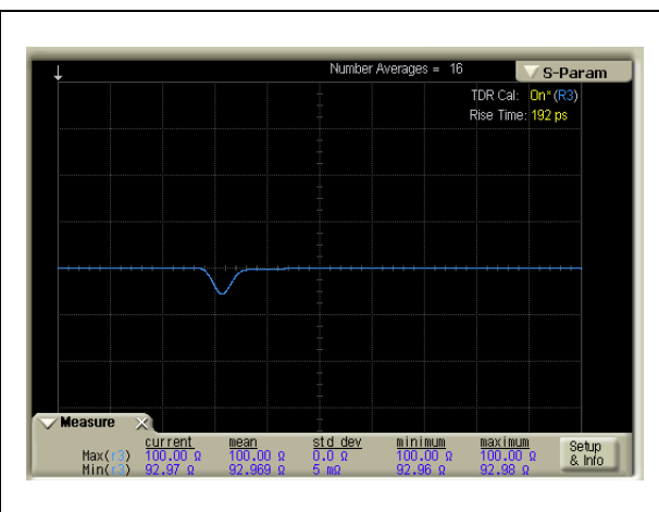
Figure 15. TDR measurement
