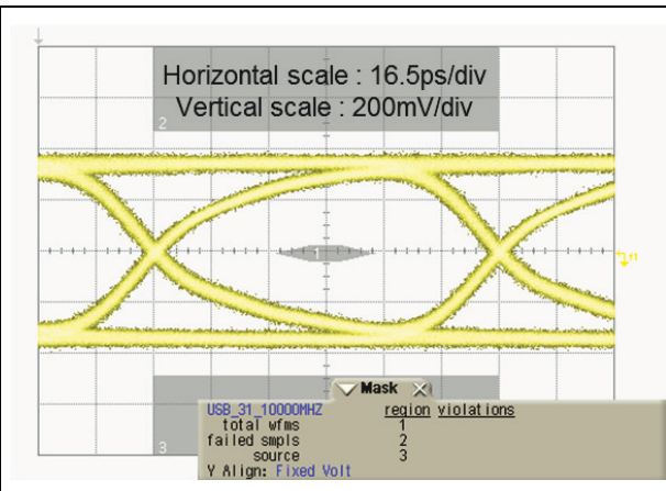
Figure 11. Eye diagram - USB 3.1 mask at 10.0 Gbps per channel (with HSP051-4N10)
