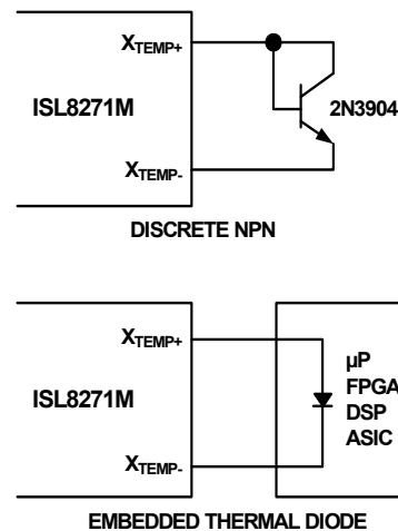
FIGURE 28. EXTERNAL TEMPERATURE MONITORING
