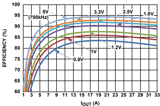
FIGURE 7. EFFICIENCY vs OUTPUT CURRENT AT V_{IN} = 12\text{V} AND f_{SW} = 533\text{kHz} FOR VARIOUS OUTPUT VOLTAGES
