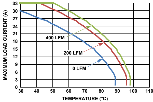
FIGURE 25. 12V_{\text{IN}} TO 5V_{\text{OUT}} , 700kHz
