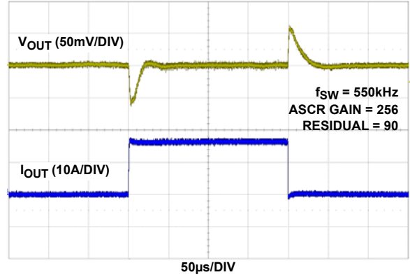
FIGURE 10. LOAD TRANSIENT RESPONSE AT V_{IN} = 12\text{V} , V_{OUT} = 1\text{V} WITH DEFAULT ASCR PARAMETERS
