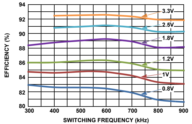
FIGURE 4. EFFICIENCY vs SWITCHING FREQUENCY AT V_{IN} = 5\text{V} AND I_{OUT} = 33\text{A} FOR VARIOUS OUTPUT VOLTAGES
