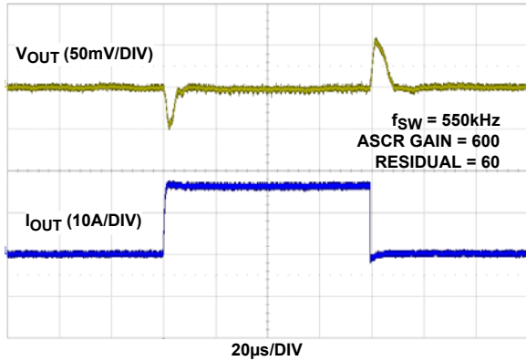
FIGURE 9. LOAD TRANSIENT RESPONSE AT V_{IN} = 12\text{V} , V_{OUT} = 1\text{V} WITH HIGH BANDWIDTH ASCR PARAMETER
