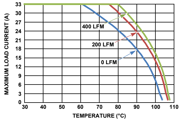
FIGURE 16. 12V_{\text{IN}} TO 1V_{\text{OUT}}
