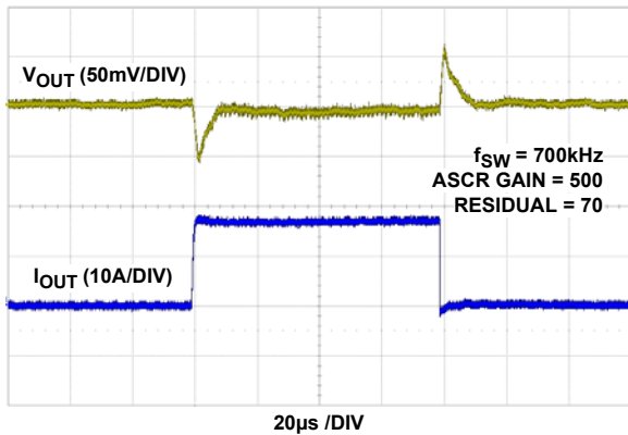
FIGURE 11. LOAD TRANSIENT RESPONSE AT V_{IN} = 12\text{V} , V_{OUT} = 2.5\text{V} WITH HIGH BANDWIDTH ASCR PARAMETERS
