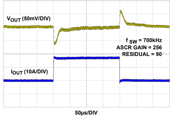
FIGURE 12. LOAD TRANSIENT RESPONSE AT V_{IN} = 12\text{V} , V_{OUT} = 2.5\text{V} WITH DEFAULT ASCR PARAMETERS
