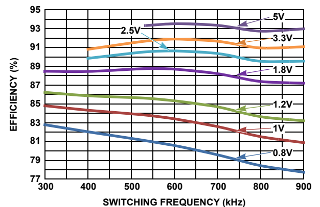
FIGURE 8. EFFICIENCY vs SWITCHING FREQUENCY AT V_{IN} = 12\text{V} AND I_{OUT} = 33\text{A} FOR VARIOUS OUTPUT VOLTAGES
