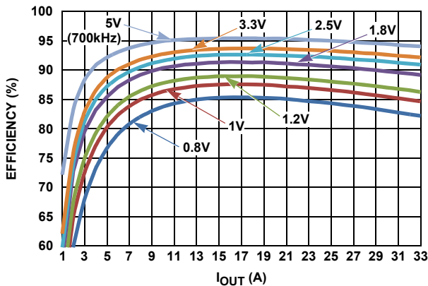
FIGURE 5. EFFICIENCY vs OUTPUT CURRENT AT V_{IN} = 9\text{V} AND f_{SW} = 533\text{kHz} FOR VARIOUS OUTPUT VOLTAGES
