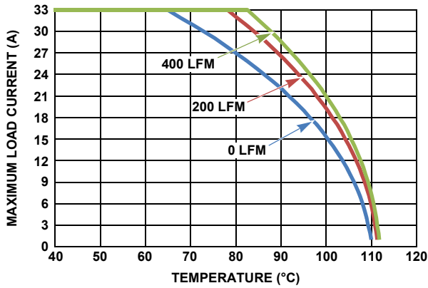
FIGURE 15. 5V_{\text{IN}} TO 1V_{\text{OUT}}
