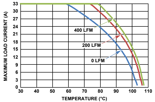
FIGURE 18. 12V_{\text{IN}} TO 1.2V_{\text{OUT}}
