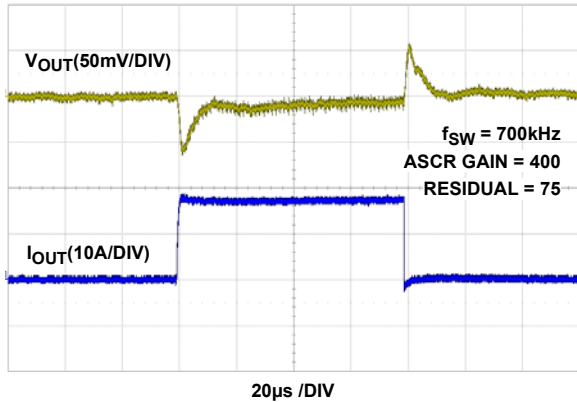
FIGURE 13. LOAD TRANSIENT RESPONSE AT V_{IN} = 12\text{V} , V_{OUT} = 3.3\text{V} WITH HIGH BANDWIDTH ASCR PARAMETERS
