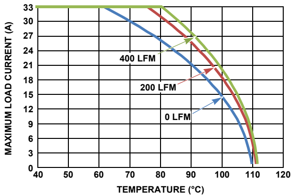
FIGURE 17. 5V_{\text{IN}} TO 1.2V_{\text{OUT}}
