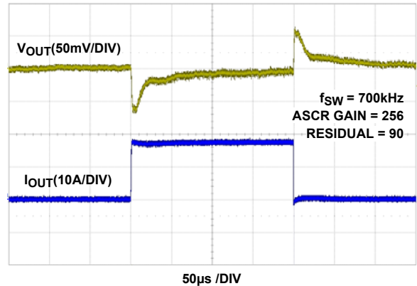
FIGURE 14. LOAD TRANSIENT RESPONSE AT V_{IN} = 12\text{V} , V_{OUT} = 3.3\text{V} WITH DEFAULT ASCR PARAMETERS
