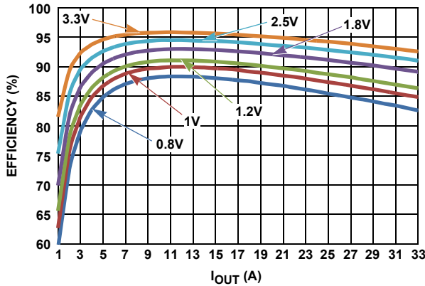
FIGURE 3. EFFICIENCY vs OUTPUT CURRENT AT V_{IN} = 5\text{V} AND f_{SW} = 533\text{kHz} FOR VARIOUS OUTPUT VOLTAGES
