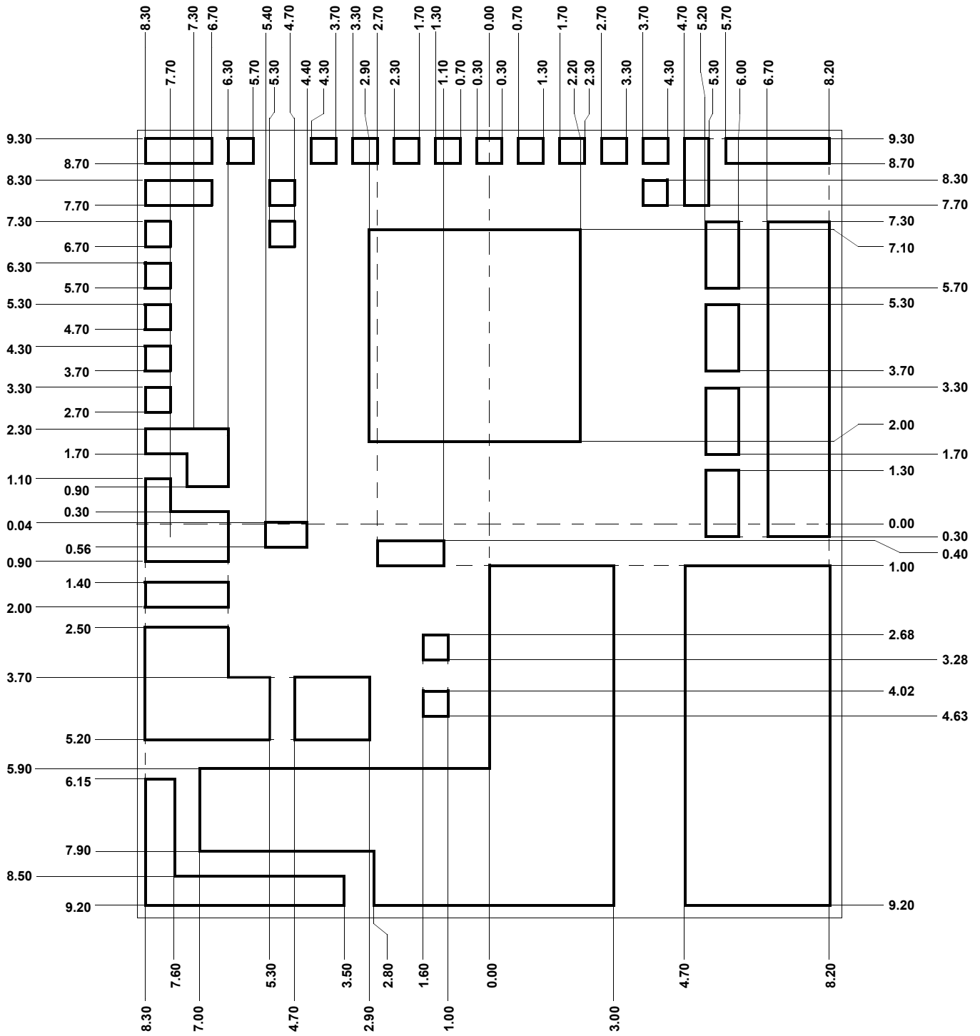
TYPICAL PCB LAND PATTERN (For Reference)
