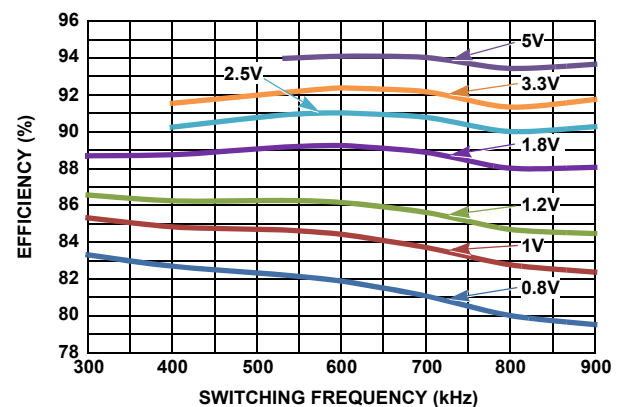
FIGURE 6. EFFICIENCY vs SWITCHING FREQUENCY AT V_{IN} = 9\text{V} AND I_{OUT} = 33\text{A} FOR VARIOUS OUTPUT VOLTAGES
