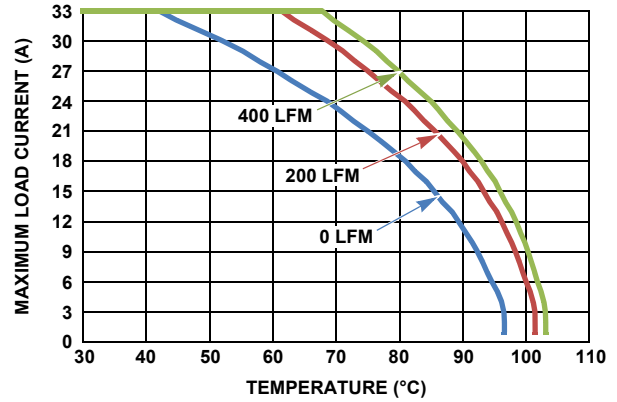
FIGURE 22. 12V_{\text{IN}} TO 2.5V_{\text{OUT}}
