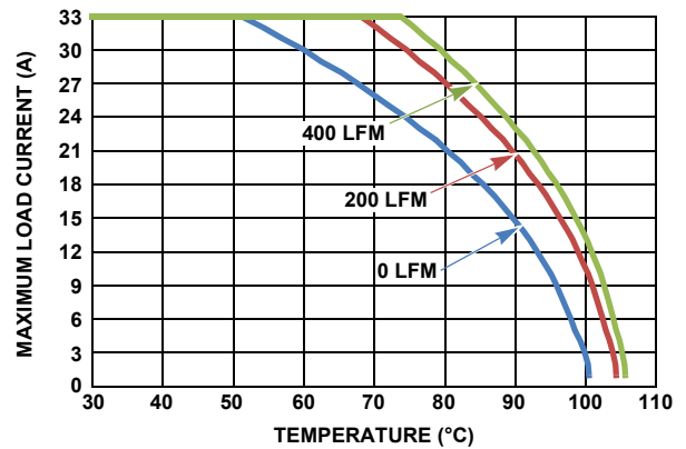
FIGURE 20. 12V_{\text{IN}} TO 1.8V_{\text{OUT}}
