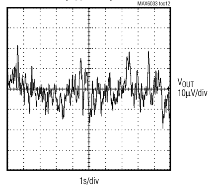
0.1Hz TO 10Hz OUTPUT NOISE ( V_{OUT} = 5V )
