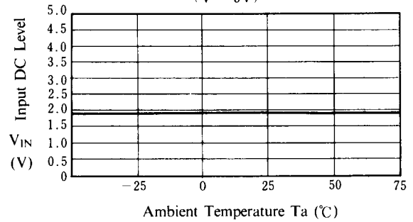
Input DC Level vs. Ta
