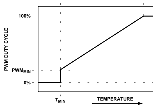
Figure 49. PWM MIN Determines Minimum PWM Duty Cycle
