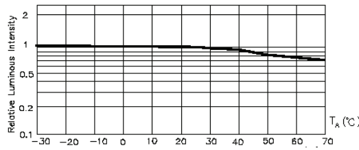
Fig.5 Luminous Intensity at I_f = 20\text{mA} vs. Ambient Temperature
