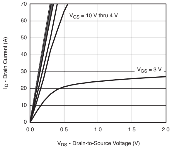
V_{GS} = 10 V thru 4 V V_{GS} = 3 V Output Characteristics
